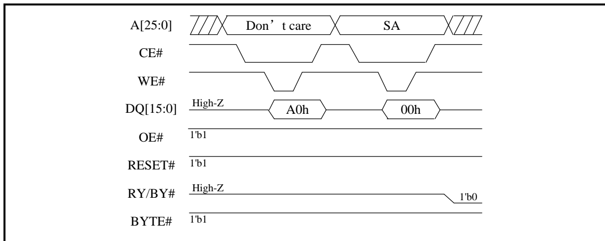
Figure 64. PPB Program (word mode)
