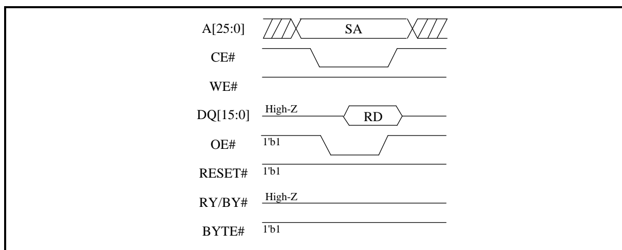
Figure 70. DYB Read(word mode)
