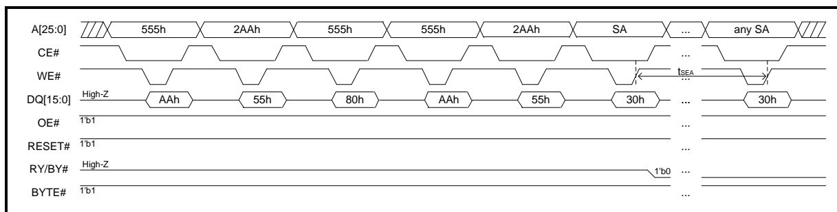
Figure 15. Sector Erase (word mode)
