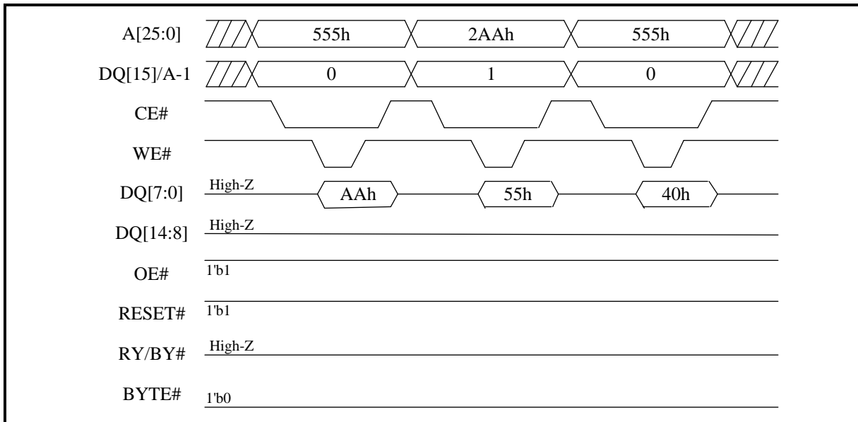
Figure 46. Lock Register Enter (byte mode)
