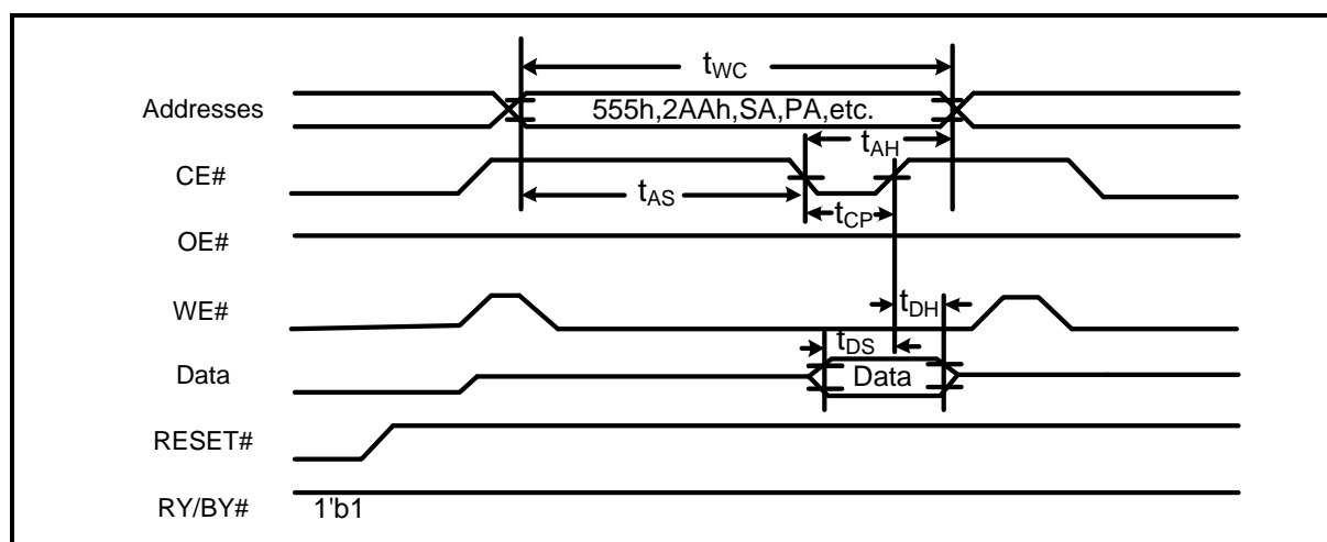
Figure 91. CE# Controlled Write Operation Timings
