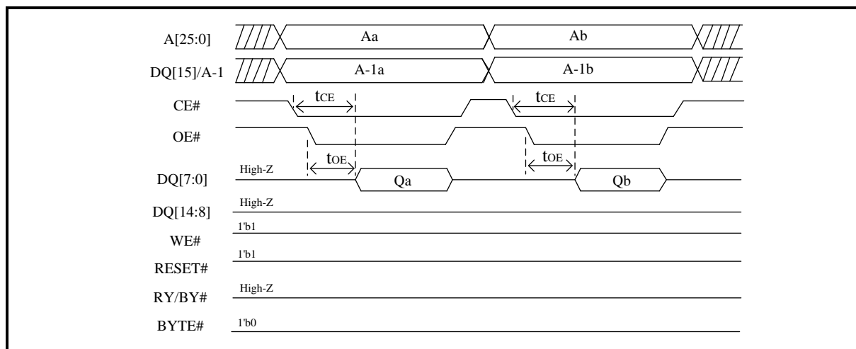
Figure 5. read function (byte mode)
