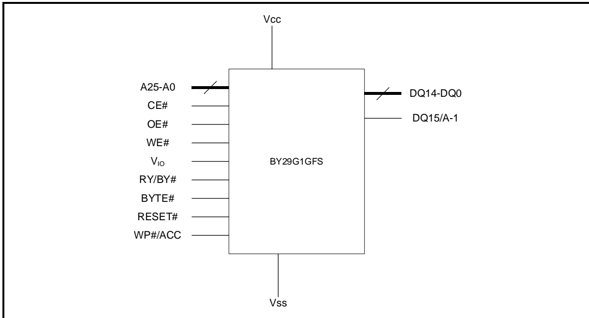
Figure 1. Logic diagram
