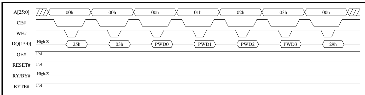
Figure 83. Password Unlock (word mode)
