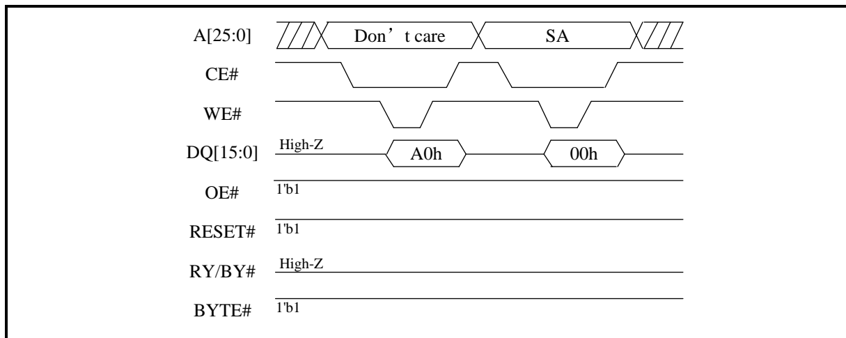
Figure 72. DYB Set (word mode)
