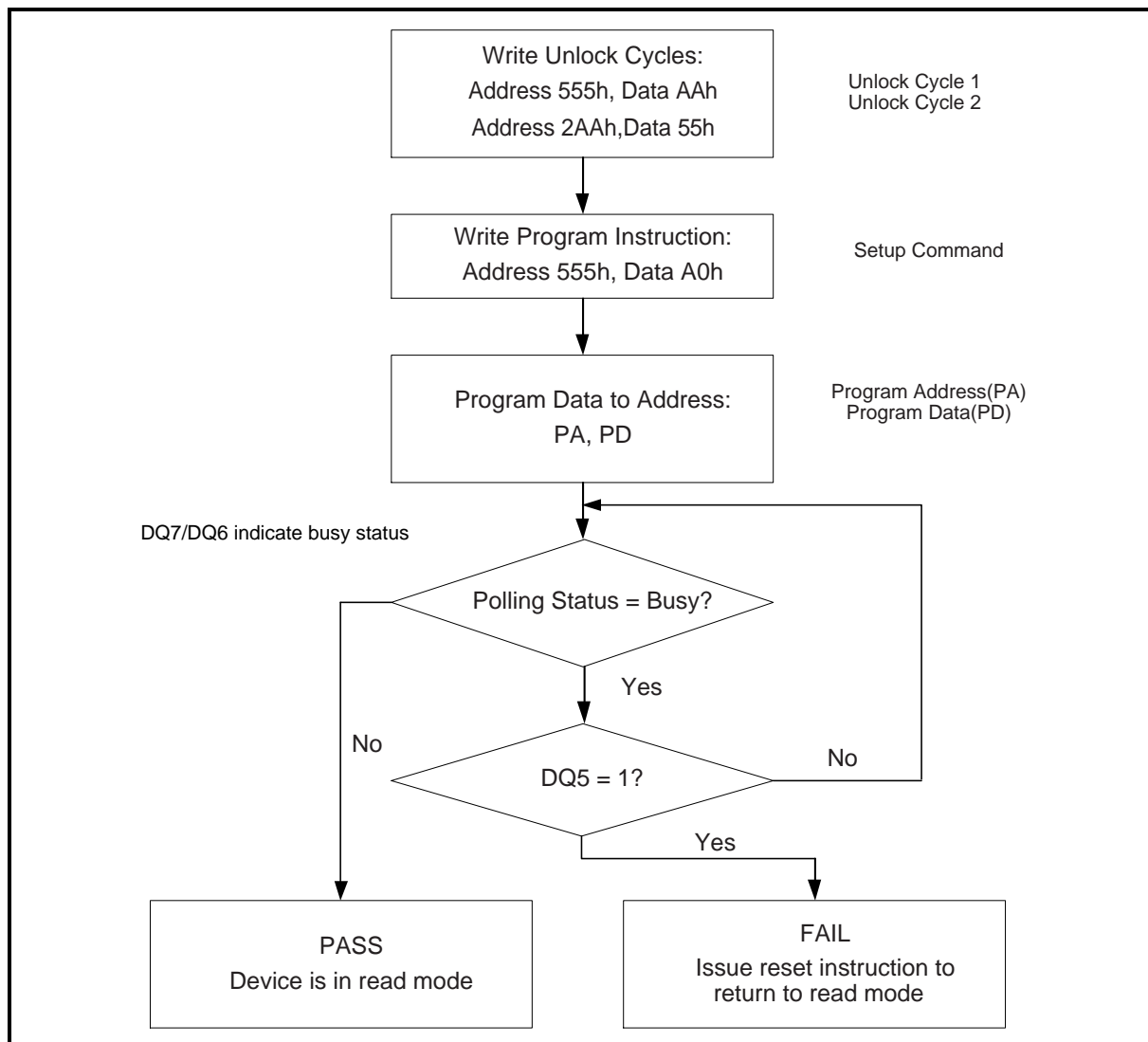
Figure 8. Single Word Program
