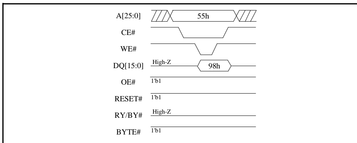
Figure 42. CFI query (word mode)
