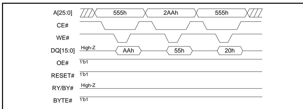
Figure 28. Unlock Bypass Entry (word mode)
