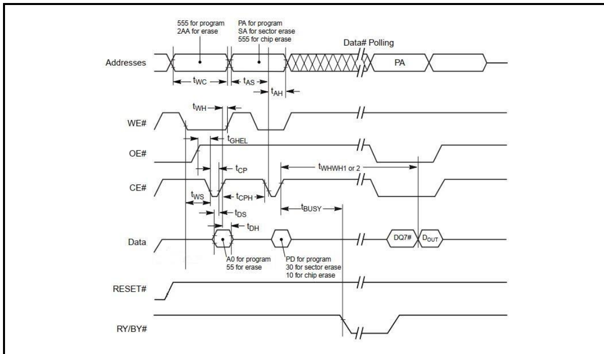
Figure 99. Alternate CE# Controlled Write (Erase/Program) Operation Timings
