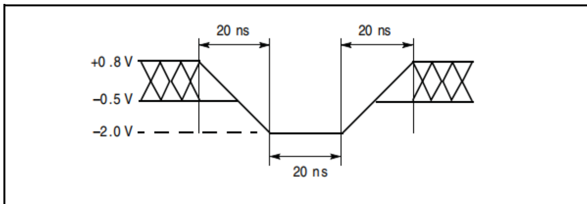
Figure 85. Maximum Negative Overshoot Waveform
