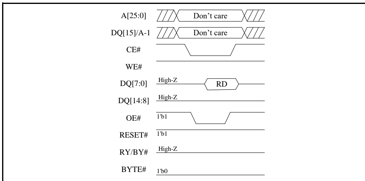
Figure 56. PPB Lock Bit Set Read (byte mode)
