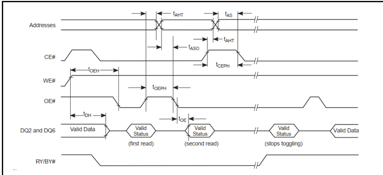
Figure 97. Toggle Bit Timings (During Embedded Algorithms)
