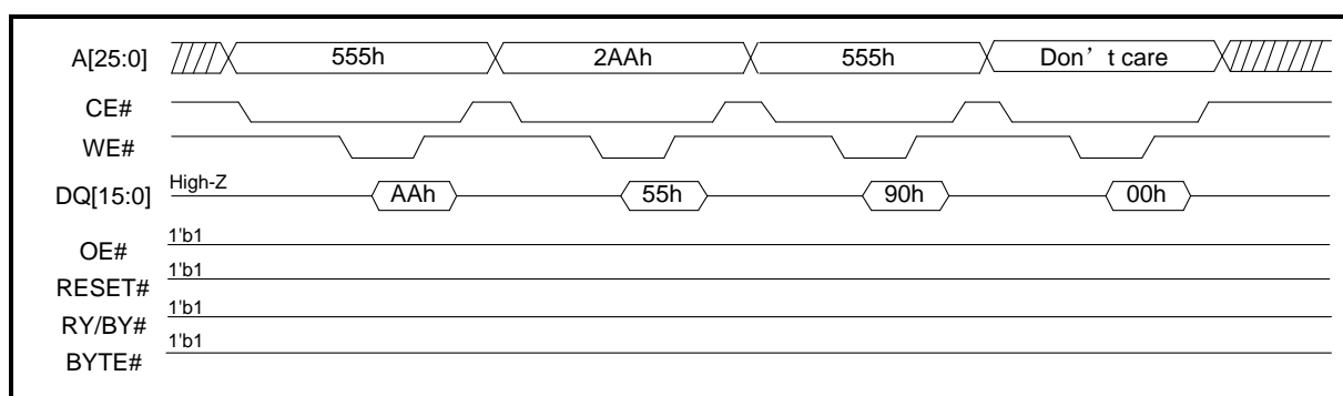
Figure 34. Secured Silicon Sector Exit (word mode)
