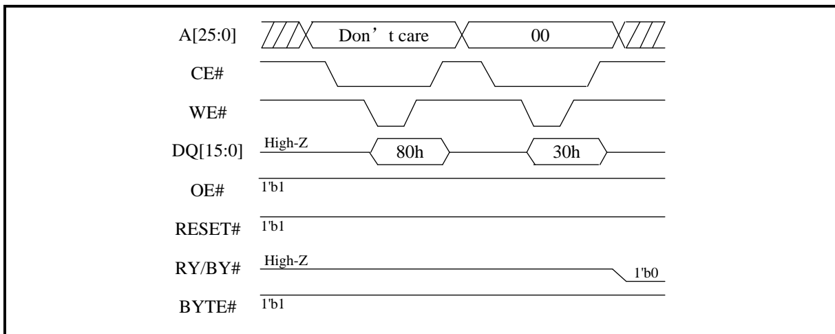
Figure 66. PPB All Erase (word mode)
