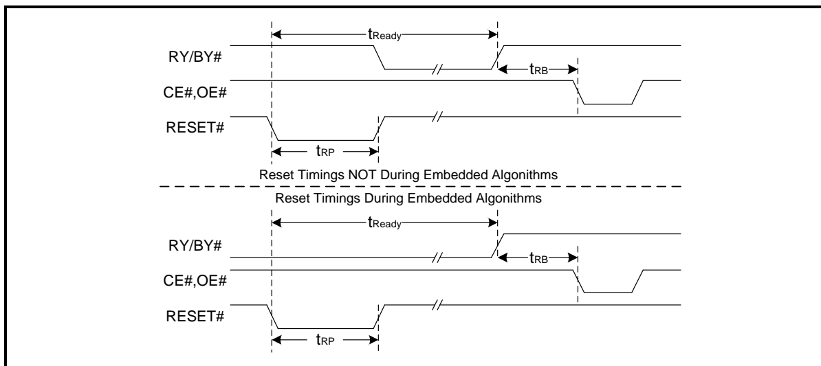
Figure 100.Reset Timings
