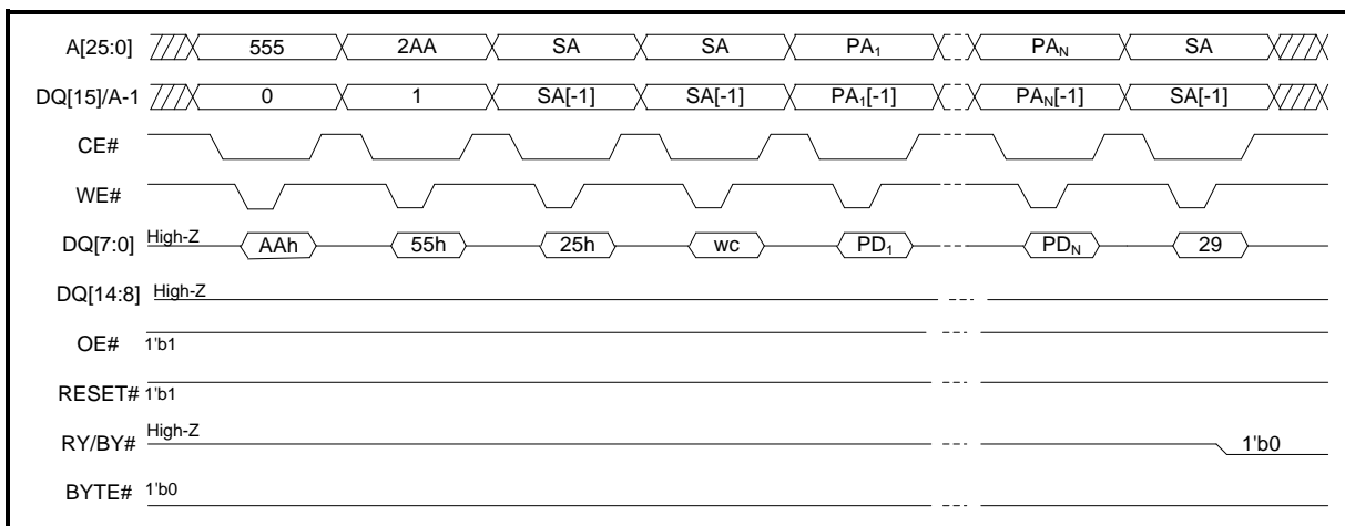
Figure 13. Write Buffer Programming (byte mode)
