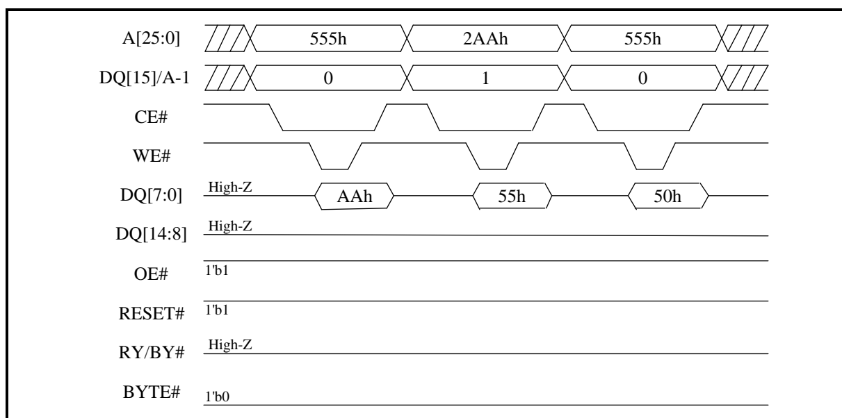
Figure 54. PPB Lock Bit Set Enter (byte mode)
