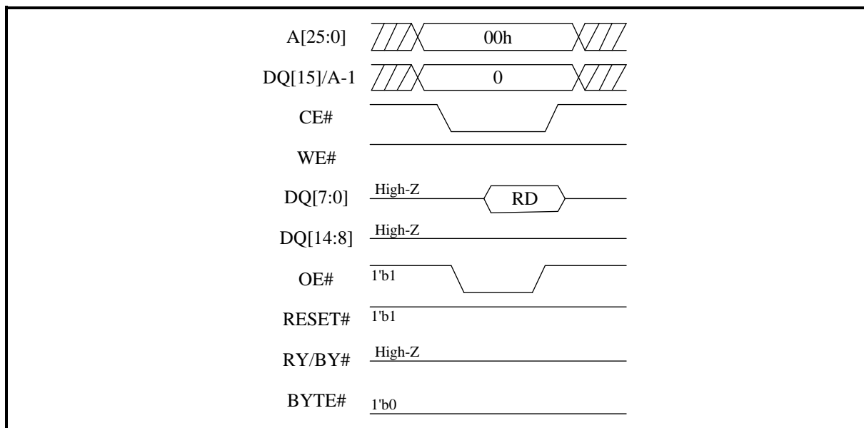
Figure 48. Lock Register Read (byte mode)
