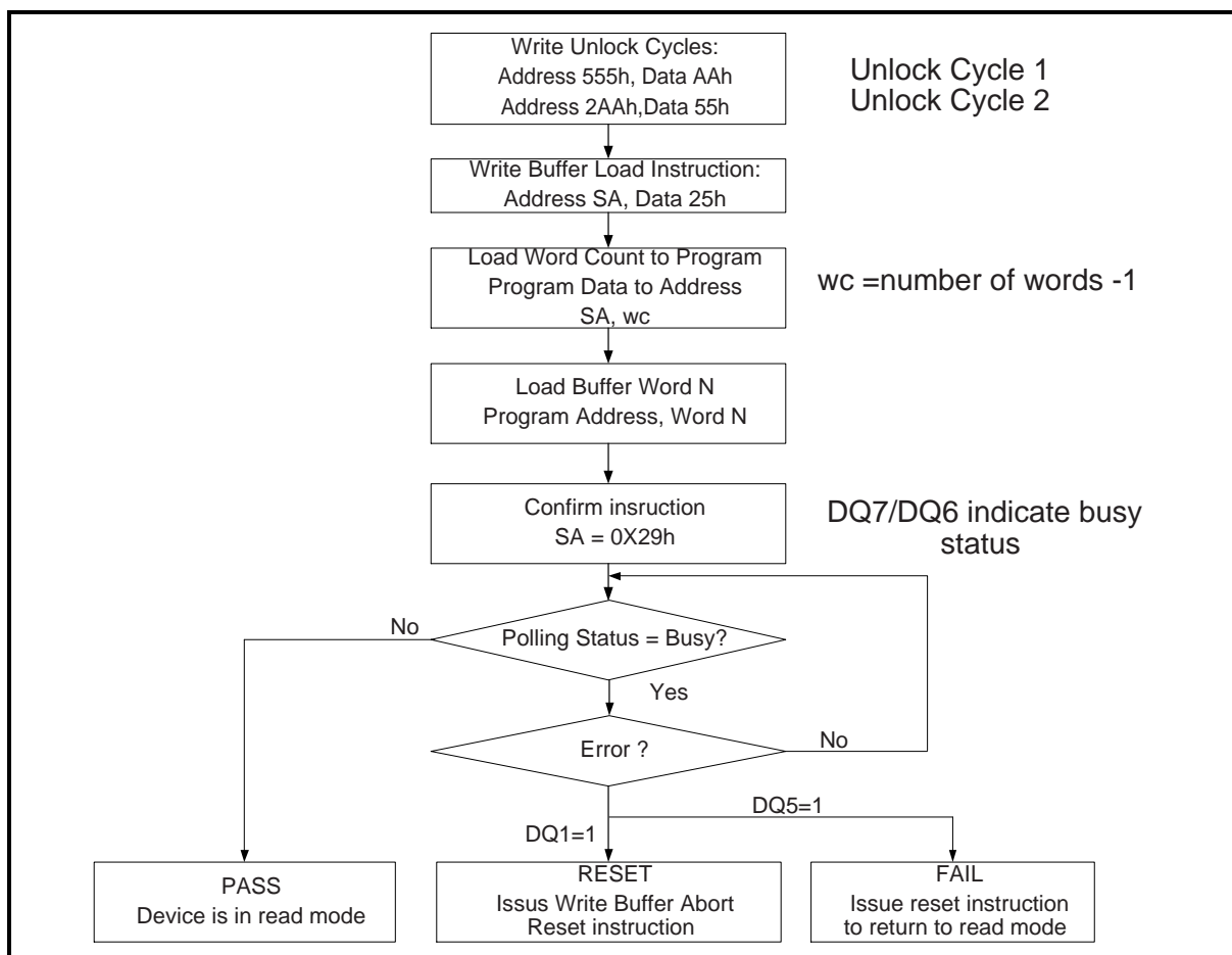
Figure 11. Write Buffer Programming Operation
