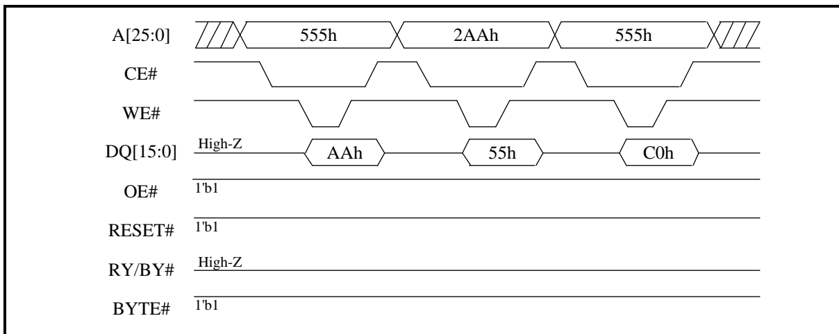
Figure 60. PPB Enter (word mode)
