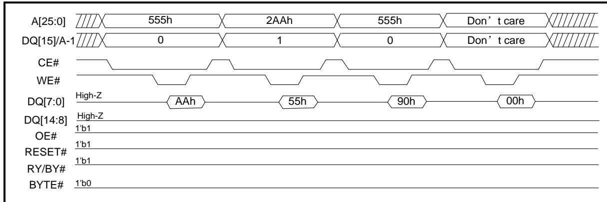
Figure 35. Secured Silicon Sector Exit (byte mode)
